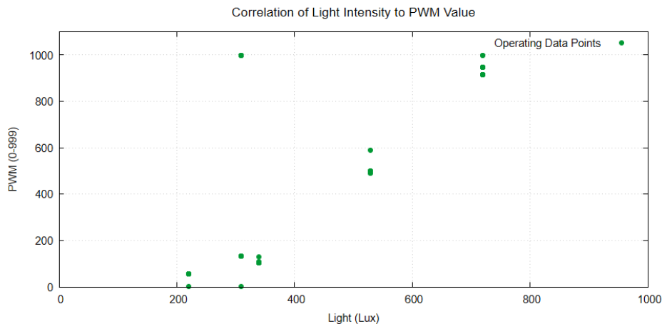
Figure 15: Korelasi Cahaya terhadap PWM.
