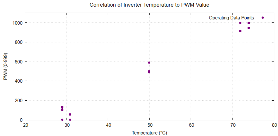
Figure 14: Korelasi Suhu terhadap PWM.
