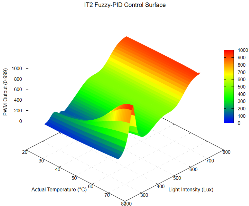
Figure 16: Representasi 3D Control Surface dari algoritma IT2 Fuzzy-PID.
